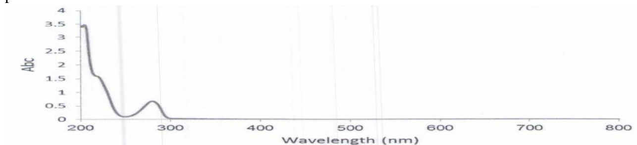
Fig-11. UV-Visible absorption spectra of Dopamine in the present of EM wave in the frequency 200HZ. The maximum absorption wave length is 280nm; the time of exposure is 60 min and the enzyme temperature 37°C .
