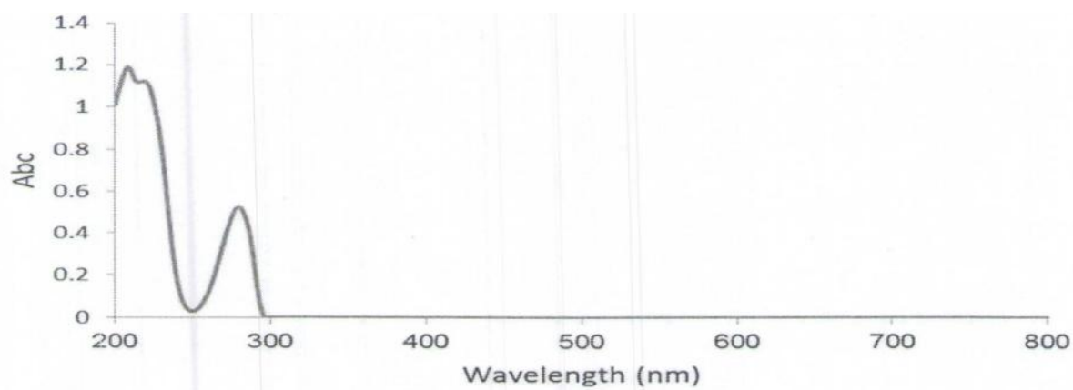
Fig-18. UV-Visible absorption spectra of Dopamine in the presence of EM wave in the frequency 1KHZ.
