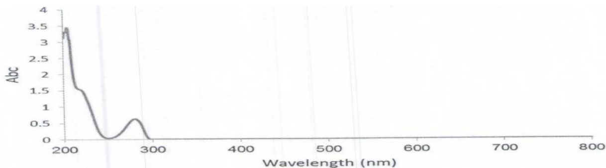
Fig-19. UV-Visible absorption spectra of Dopamine in the presence of EM wave in the frequency 1KHZ.
