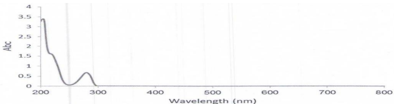
Fig-5. uv-visible absorption spectra of Dopamine in the present of EM wave in the frequency 100HZ.
