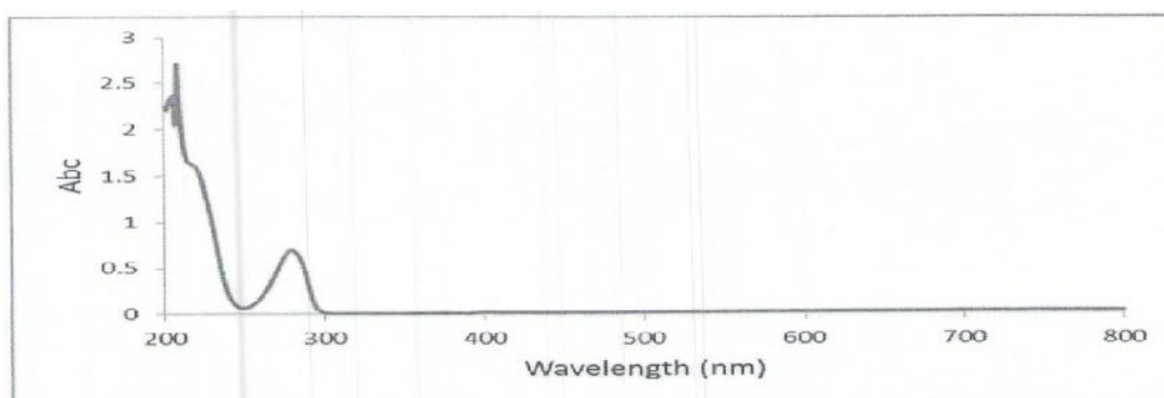
Fig-2. Far uv-visible Dopamine absorption in the absent of EM field .
