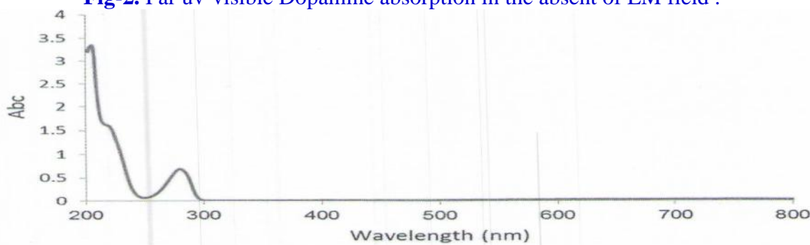
Fig-3. uv-visible Absorption spectra of Dopamine in the present of EM wave in frequency 100HZ. The maximum absorption in this wave length is 280nm; the time of exposure is 15min and the enzyme temperature is 37^{\circ}\text{C}
