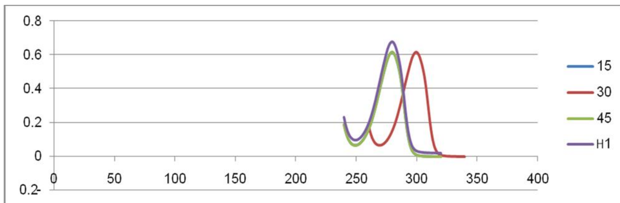
Fig-17. UV-Visible absorption spectra of Dopamine in the presence of EM wave frequency 500Hz with the time 15-60 min for comparison, the enzyme temperature again is 37°C.
